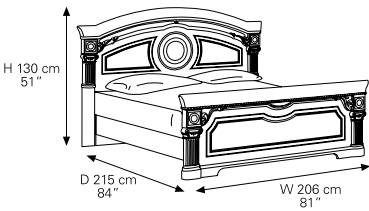
Aida bed KS cm 180 x 200/203 (mattress size) Also available cm 210 or cm 215 side rails Vol. 0,34 mc - Box 3 - Kg 72,50
